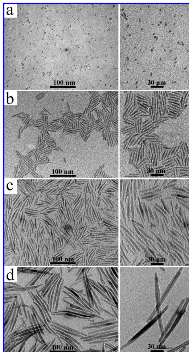
Figure 1. Low- and high-magnification (left and right panels, respectively) TEM overview of TiO 2 nanocrystals synthesized at lower OLAM/OLAC ratios. The flask, containing 0.5 mmol of TiCl 4 , 0.5 mmol of OLAC, 13 mmol of OLAM, and 3 g of ODE, was slowly heated up to 290 °C and kept at this temperature for 30 min (a). Subsequently, varying amounts of an equimolar TiCl 4 /OLAC mixture were added at a rate of 0.1 mL/min at 290 °C: (b) 2 mmol; (c) 8 mmol; (d) 20 mmol.
