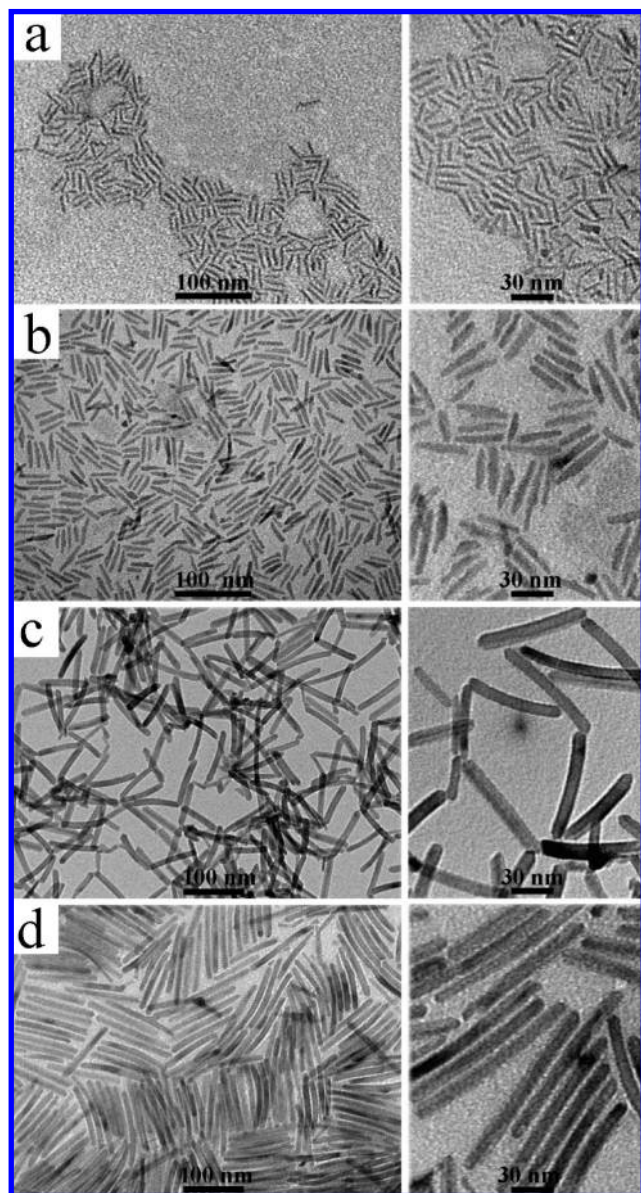
Figure 2. Low- and high-magnification (left and right panels, respectively) TEM overview of TiO 2 nanocrystals synthesized at higher OLAM/OLAC ratios. The flask, containing 0.5 mmol of TiCl 4 , 0.5 mmol of OLAC, 52 mmol of OLAM, and 3 g of ODE, was slowly heated up to 290 °C and kept at this temperature for 30 min (a). Subsequently, varying amounts of an equimolar TiCl 4 /OLAM mixture in ODE were added at a rate of 0.1 mL/min at 290 °C: (b) 2 mmol; (c) 12 mmol; (d) 20 mmol.
